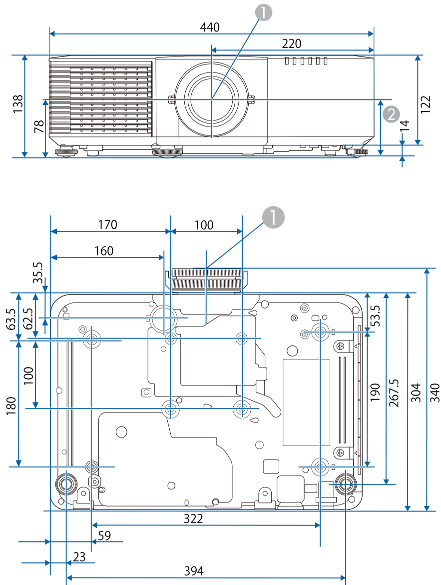
EB-L890E/EB-L895E/EB-L690E/EB-L890U/EB-L895U/EB-L790U/EB-L690U
