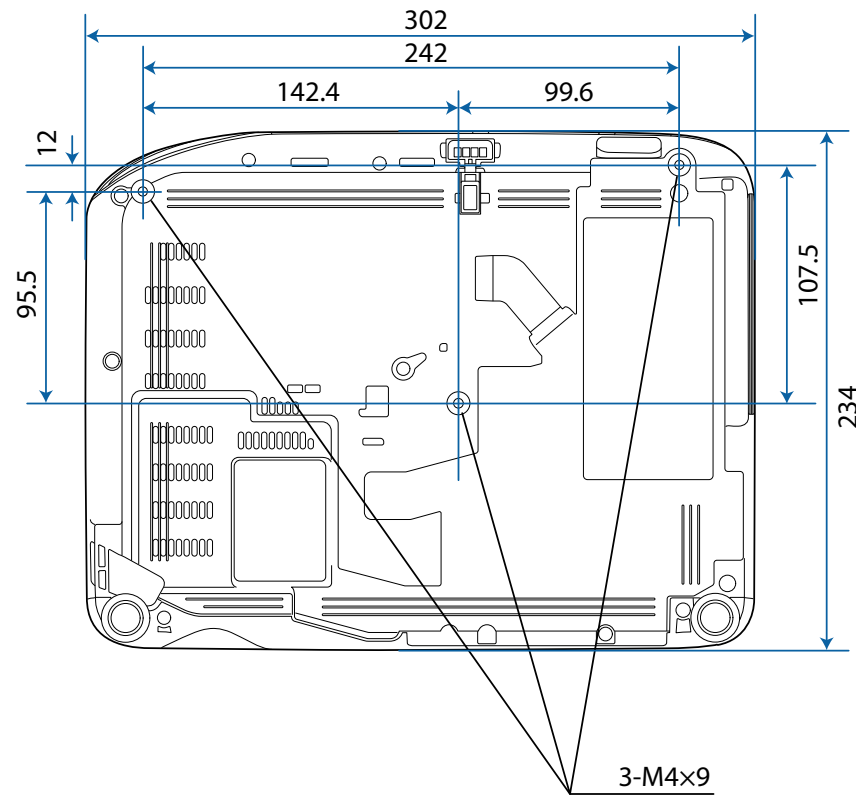
EB-E12/EB-EA12
