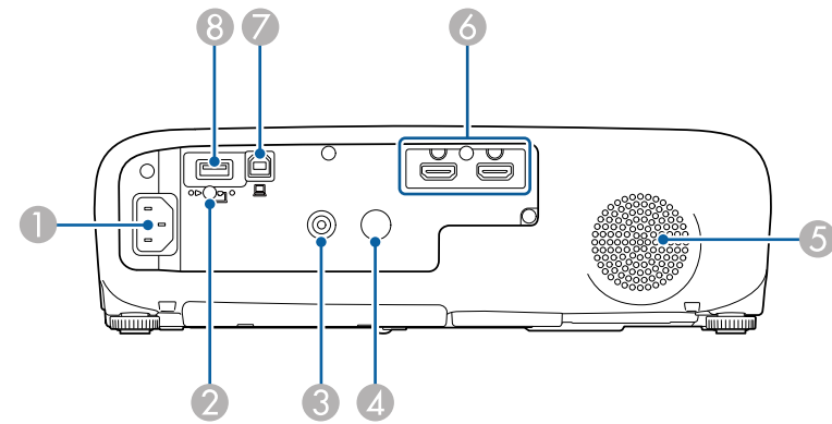
EB-W55/EB-EA55
